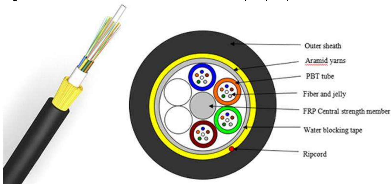
Figure 1. Cable Structure
